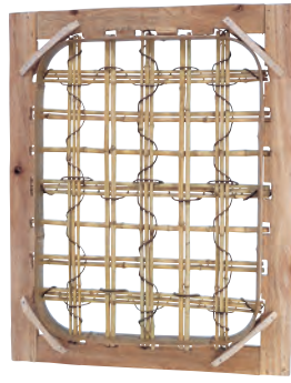
Shitajimado Bamboo
