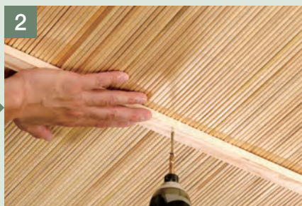
2 The wood is screwed on to the ceiling. *Be sure to screw the nail all the way into the wood.
